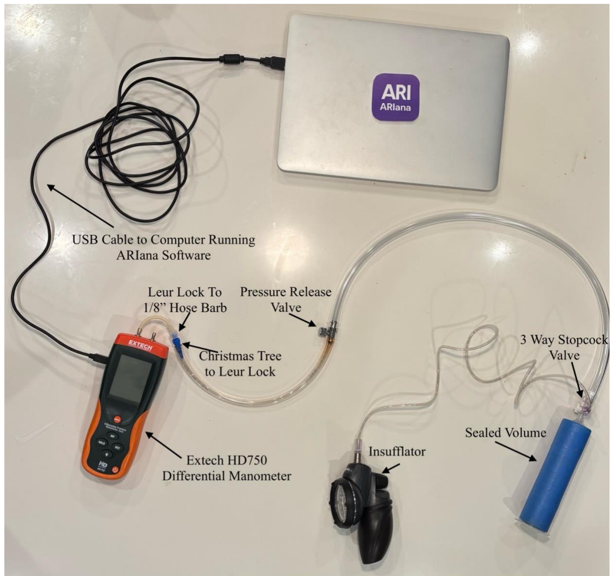
Figure 2: Simplified Setup without Mannequin
